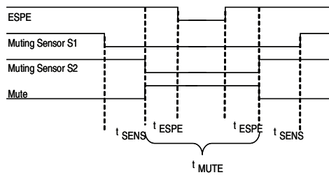
Timing for 2 Sensor T-type (standard factory supplied configuration)
