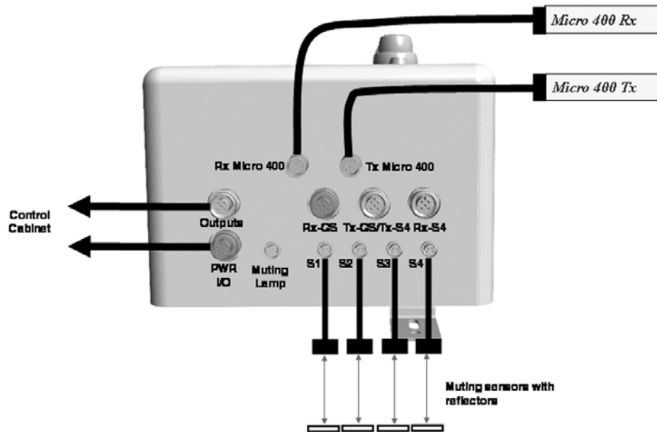
Figure 3: Wiring four sensor muting (T-Type) with GuardShield Micro 400
